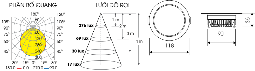
AT28 90/8W
