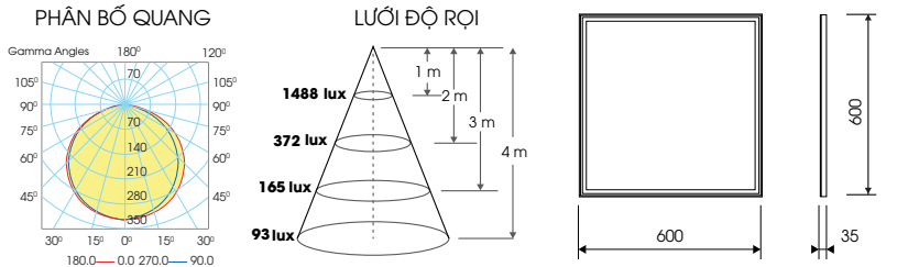
P06.UGR19.T 600x600/50W
