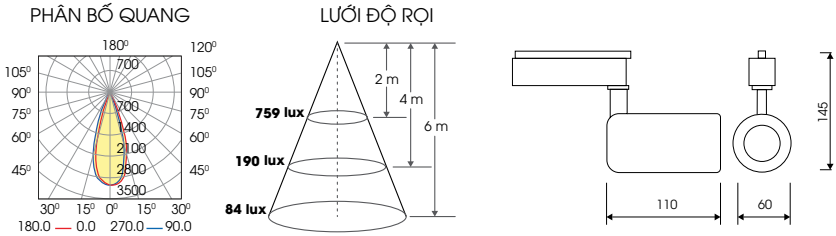
TRL05 10W
