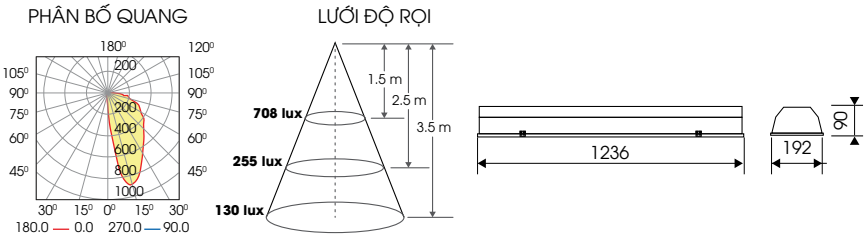
T8 CSBA/20Wx1
