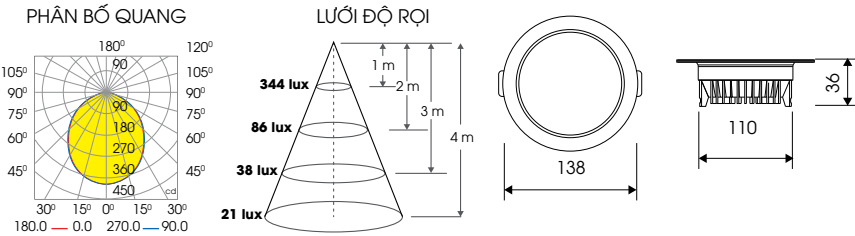
AT28 110/10W
