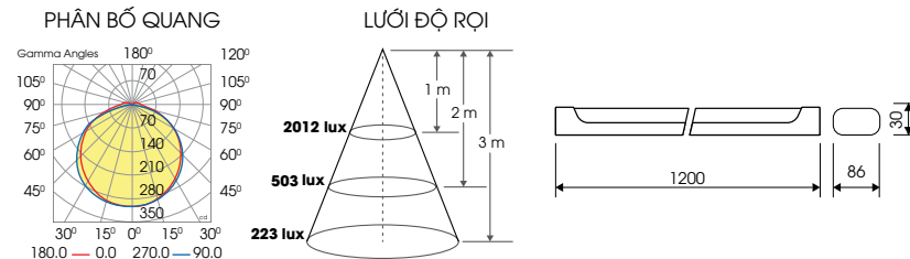
M66 1200/60W
