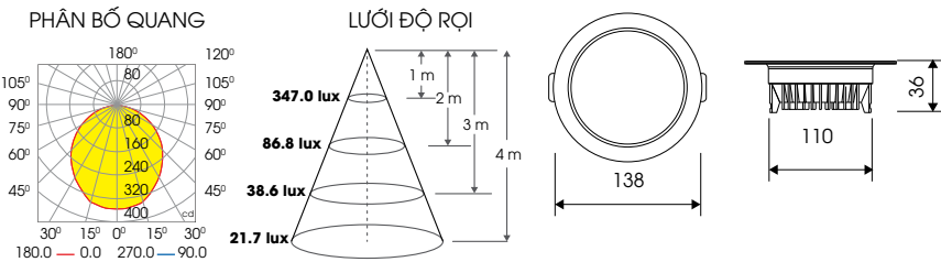
AT28 110/12W
