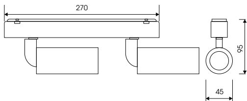
TRL08 20W
