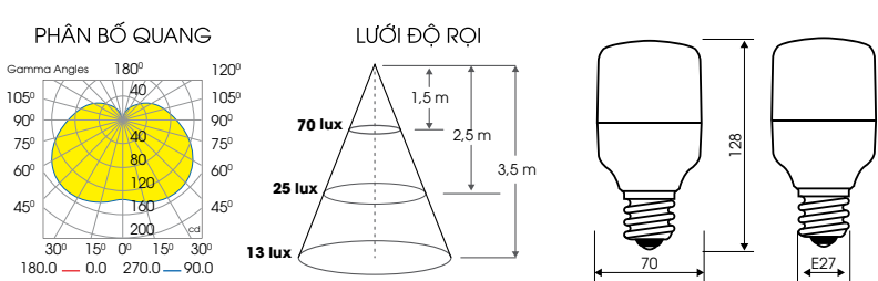
TR70N2/12W.H
