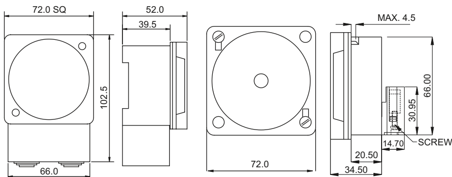
Base Mounting
