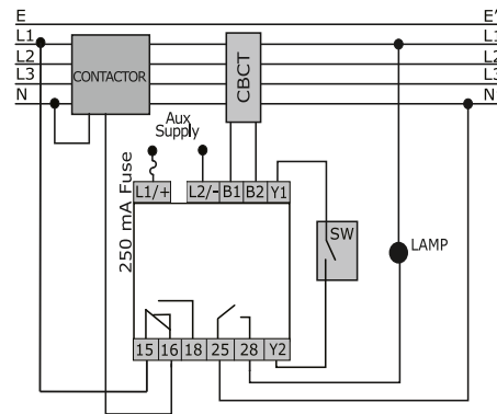
NON-FAIL SAFE MODE (CONTACTOR)
