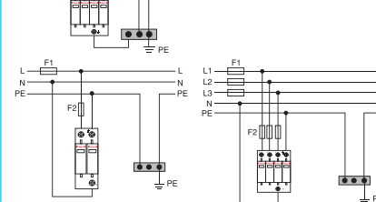
TT System HDY3N Installation Diagram
